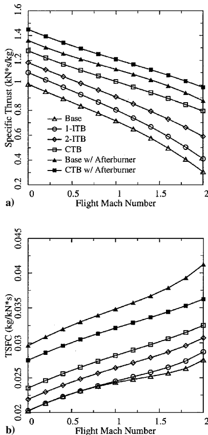
Fig. 15 Performance comparisons for turbojet engines vs flight Mach number. T_{04} = 1500 K, and T_{06} = 1900 K; \pi_c = 30 for the conventional engines; \pi_c = 60 for the turbine-burner engines.
