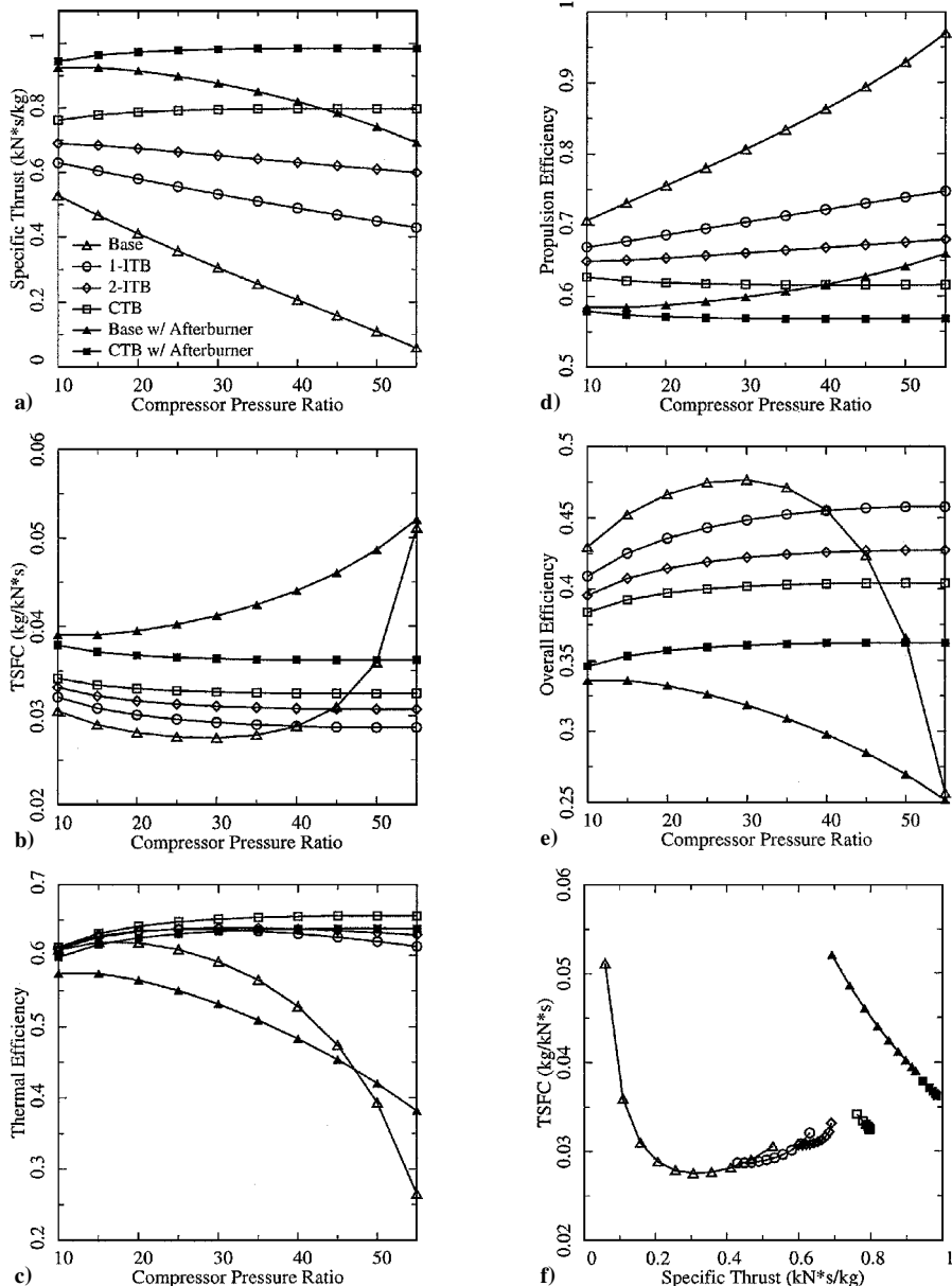
Fig. 4 Performances of turbojet engines vs compressor pressure ratio at M_\infty = 2.0 , T_{04} = 1500 K, and T_{06} = 1900 K.
